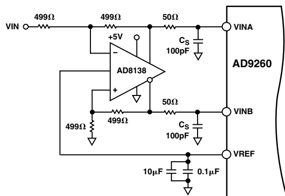
Figure 57. AD8138 Single-Ended Differential ADC Driver
