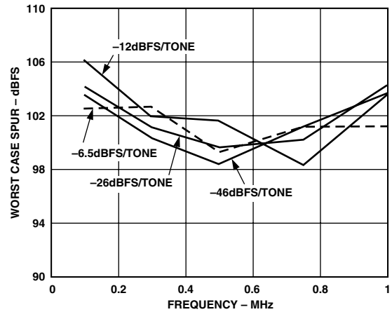
Figure 9. Dual Tone SFDR vs. Input Frequency ( F_1 = F_2 , F_1 - F_2 , Span = 10% Center Frequency, Mode = 8×)
