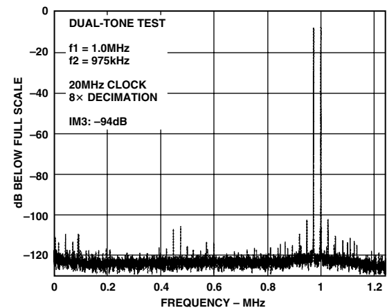
Figure 10. Two-Tone Spectral Performance of the AD9260 Given Inputs at 975 kHz and 1.0 MHz, 20 MHz Clock, 8× Decimation
