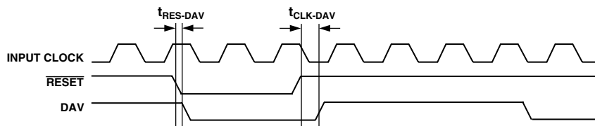
Figure 4b. \overline{RESET} Timing Diagram
